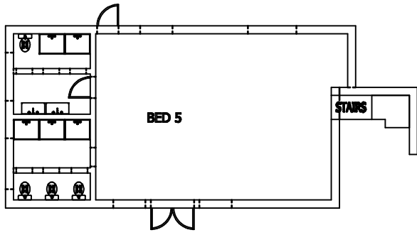
LOWER GROUND FLOOR DORM LAYOUT
